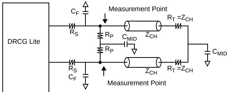
Figure 4. Output Driver
