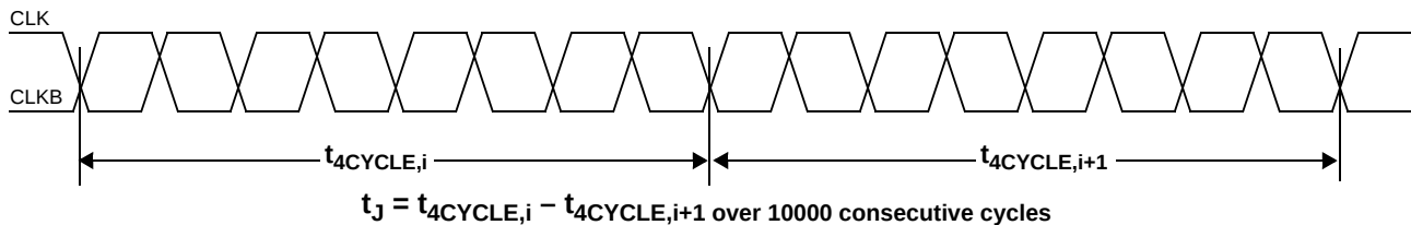
Figure 11. Short-Term Jitter
