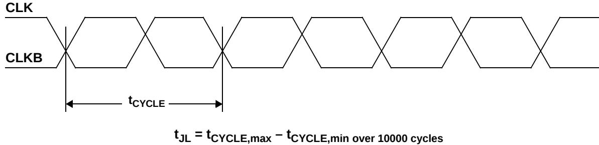
Figure 9. Long-Term Jitter
