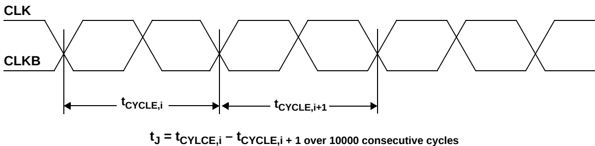
Figure 10. Cycle-to-Cycle Jitter
