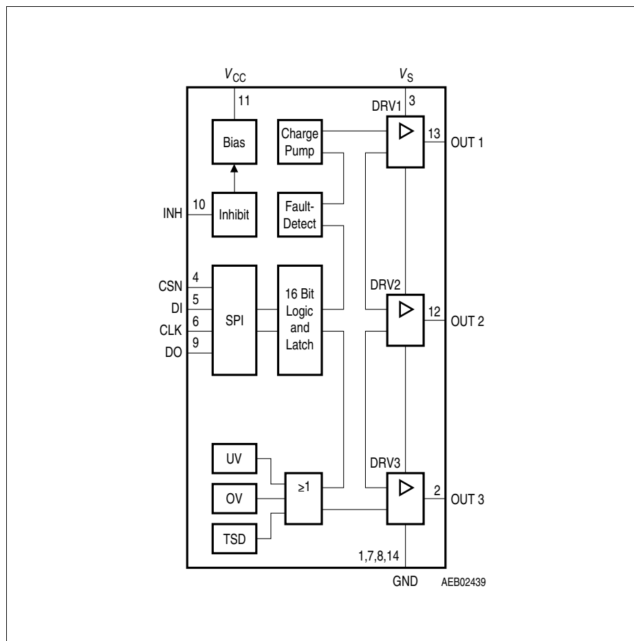
Figure 2 Block Diagram
