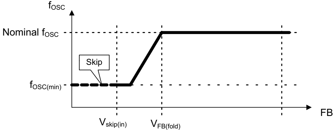
Figure 64. Frequency Foldback when the FB Voltage Decreases
