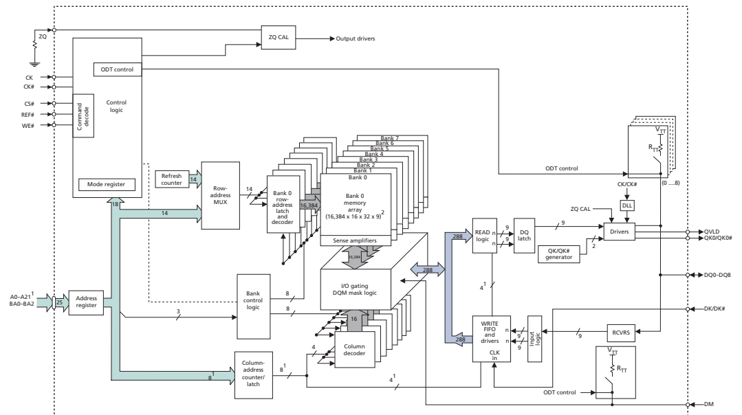
32 Meg x 18 Functional Block Diagram
