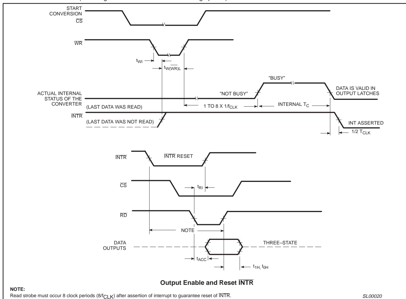
Figure 5. Timing Diagrams
