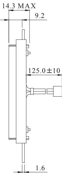
CCFL B/L
