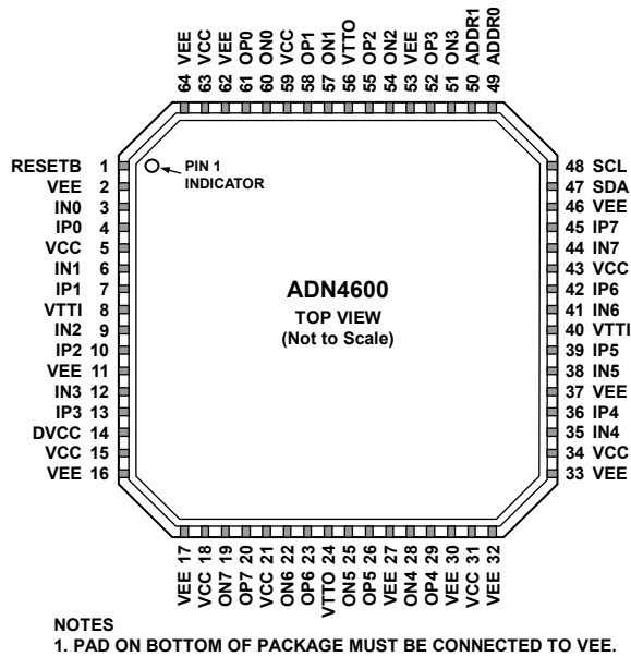
Figure 3. Pin Configuration
