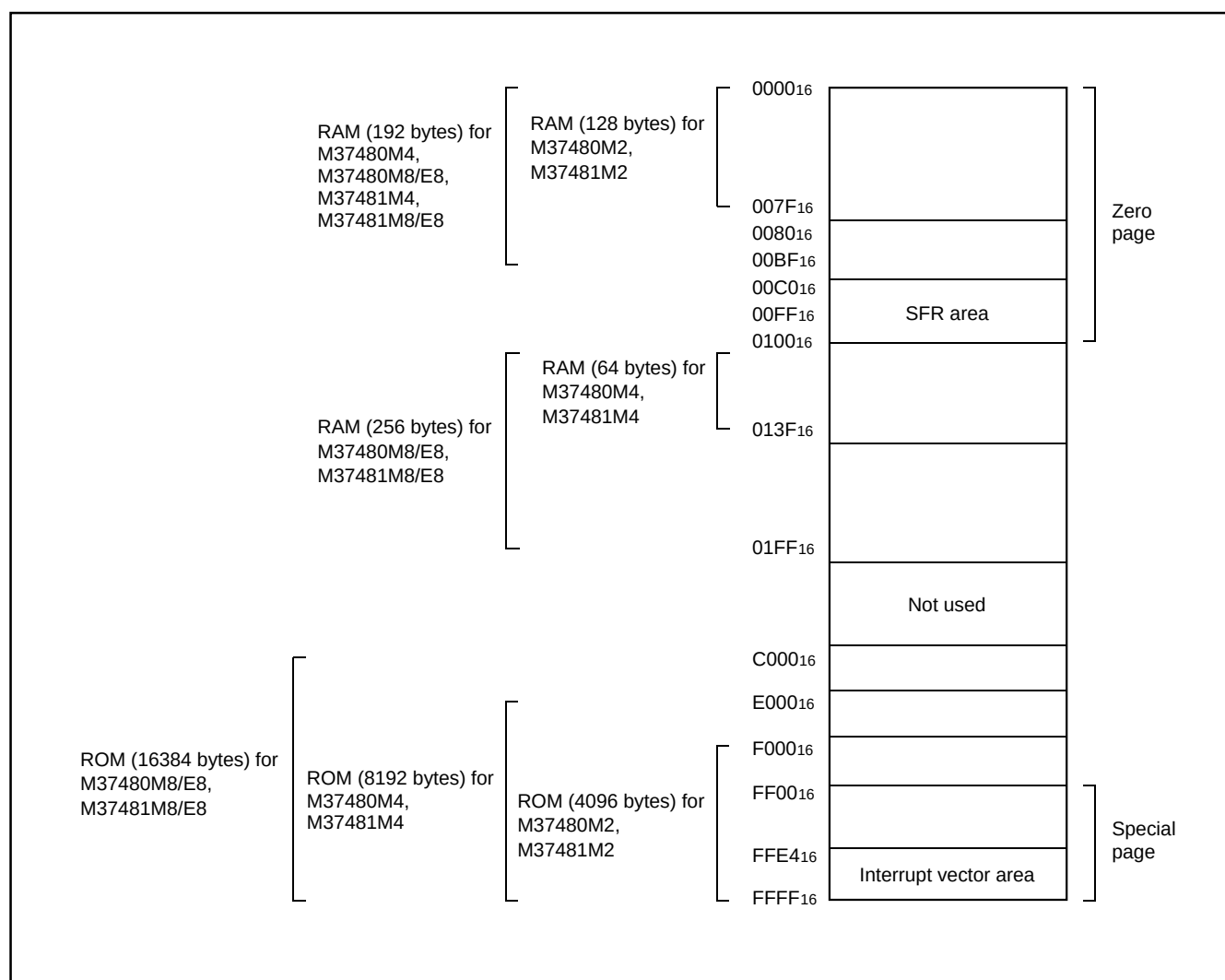
Fig. 8 Memory map
