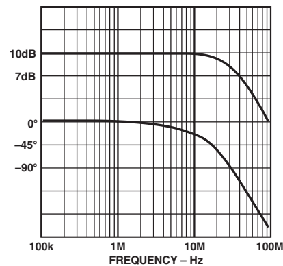
TPC 3. AD602 Frequency and Phase Response vs. Gain
