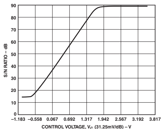
Figure 34. S/N Ratio vs. Control Voltage for Sequential Gain Control (Figure 29)
