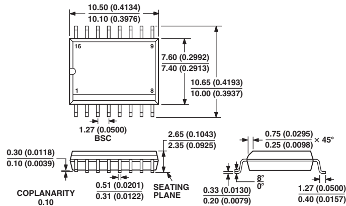
16-Lead SOIC Package (R-16)
