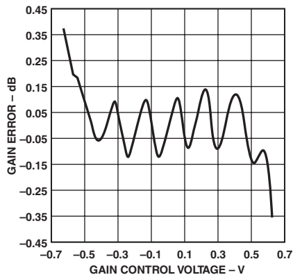
TPC 1. Gain Error vs. Gain Control Voltage
