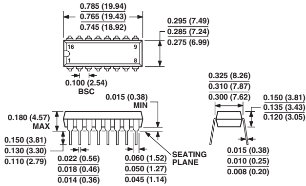
16-Lead Plastic DIP Package (N-16)
