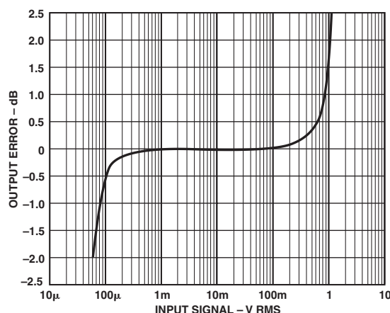
Figure 24. Using the 3 dB Offset Network, the Ripple Is Reduced
