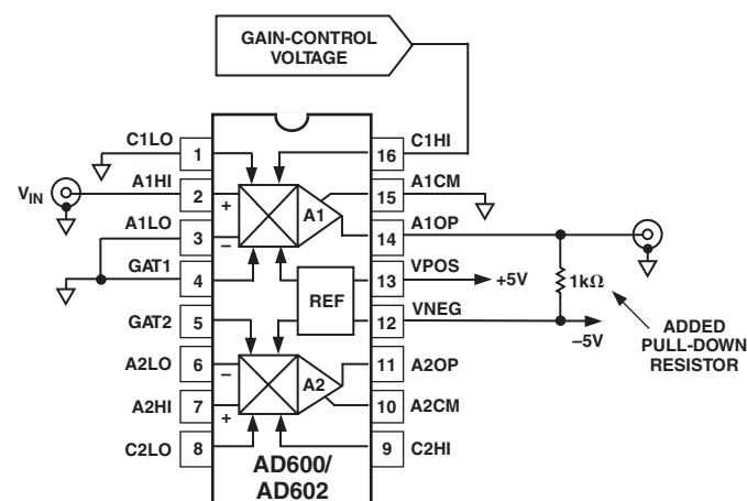
Figure 12. Adding a 1 \text{ k}\Omega Pull-Down Resistor Increases the X-AMP's Output Drive by About 5 mA. Only the A1 connections are shown for simplicity.
