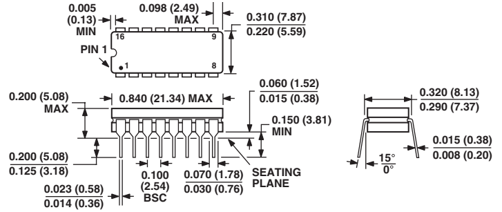
16-Lead Cerdip Package (Q-16)
