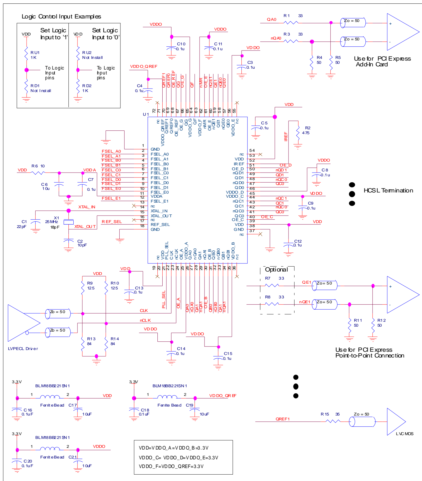
Figure 6. ICS8413S12BI Schematic Example
