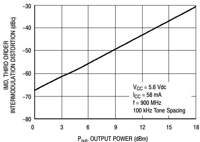
Figure 10. Third Order Intermodulation versus Output Power
