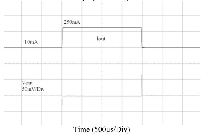
PT7M8202 (3.3V)
