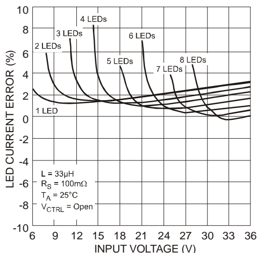
Figure 23. LED Current Deviation vs. Input Voltage
