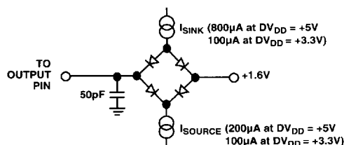
Figure 1. Load Circuit for Access Time and Bus Relinquish Time
