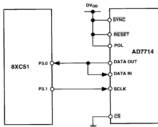
Figure 10. AD7714 to 8051 Interface
