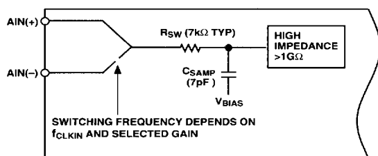
Figure 3. Unbuffered Analog Input Structure
