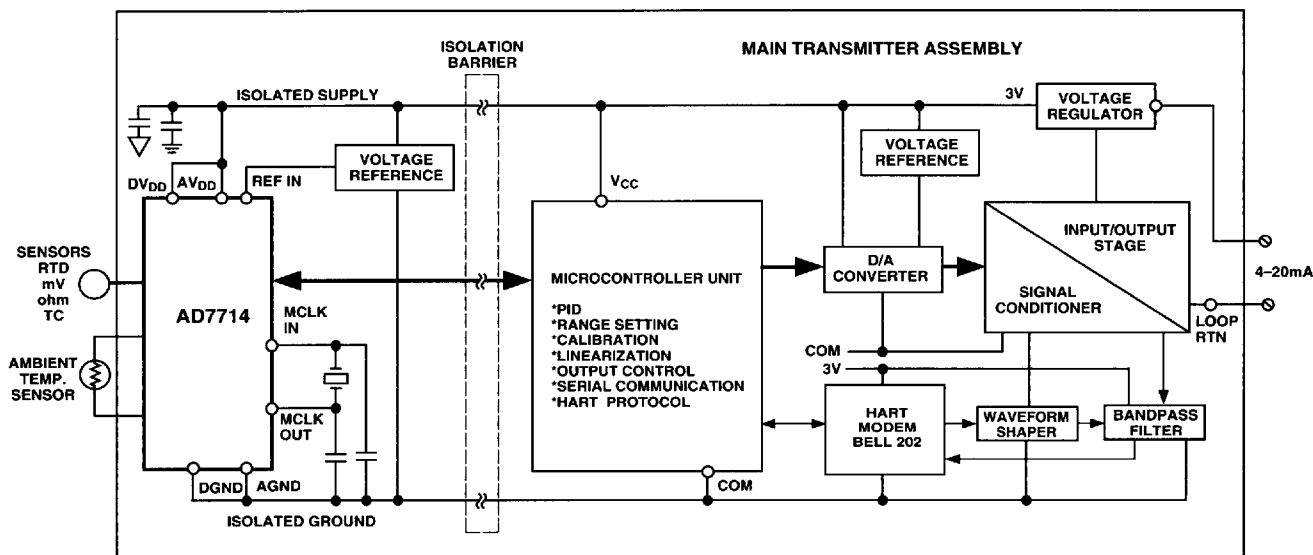
Figure 16. Smart Transmitter Using the AD7714
