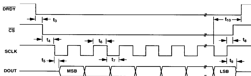
Figure 6. Read Cycle Timing Diagram (POL = 1)
