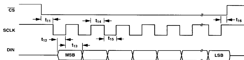
Figure 7. Write Cycle Timing Diagram (POL = 1)
