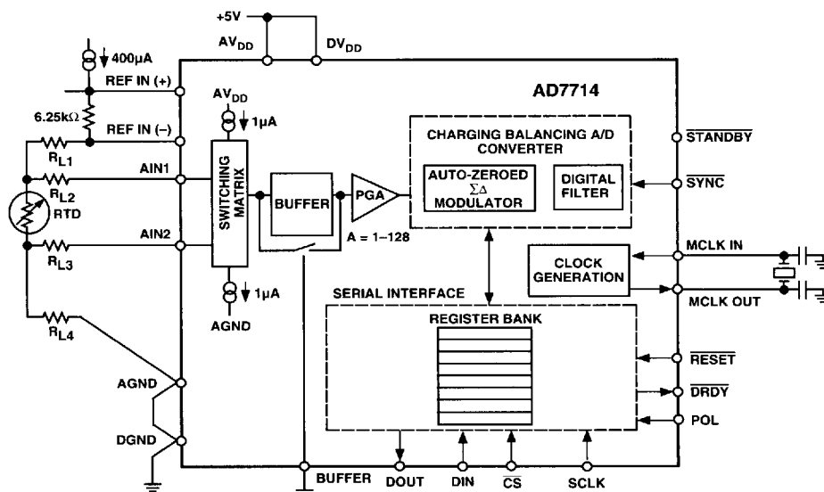
Figure 14. RTD Measurement Using the AD7714
