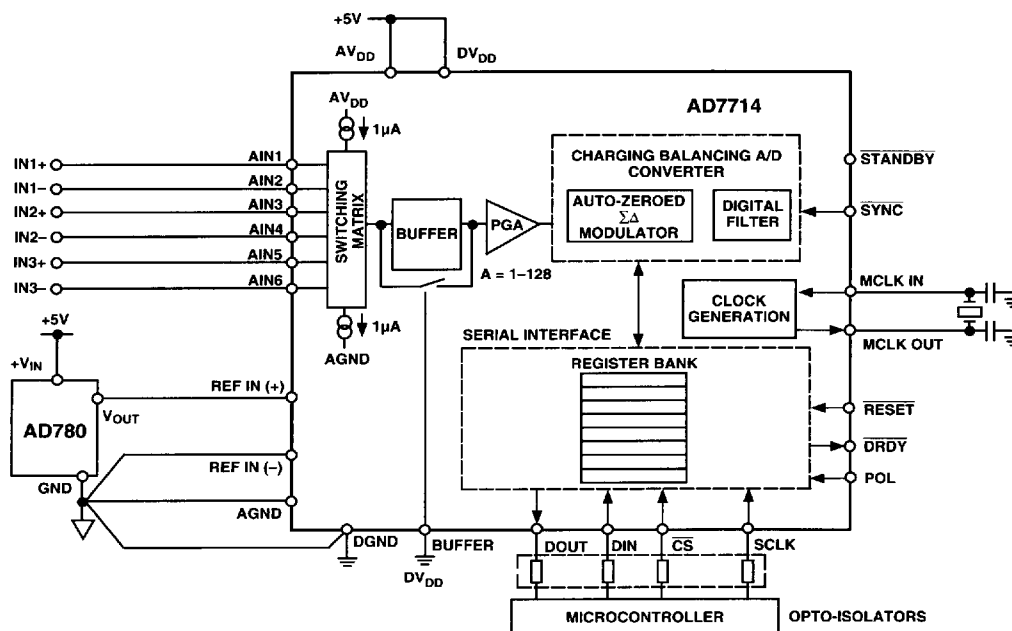
Figure 15. Data Acquisition System Using the AD7714
