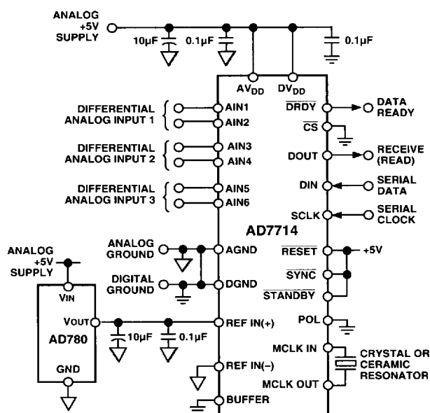
Figure 2. Basic Connection Diagram
