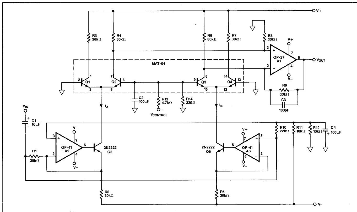
FIGURE 9: Voltage-Controlled Attenuator
