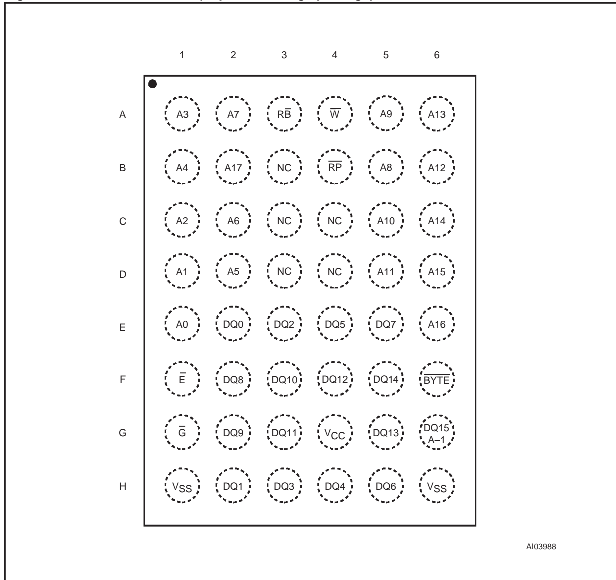
Figure 4. TFBGA Connections (Top view through package)
