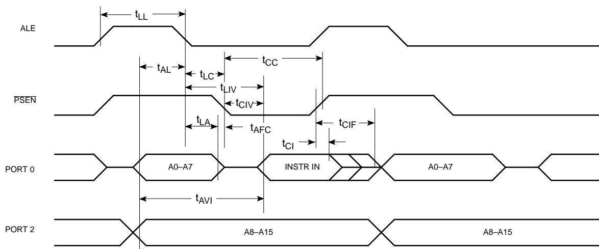
Figure 10. External Program Memory Read Cycle
