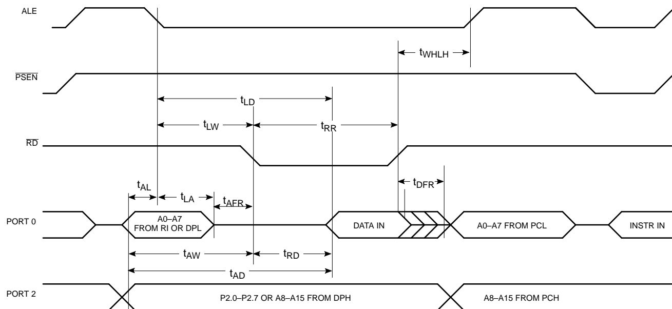
Figure 11. External Data Memory Read Cycle
