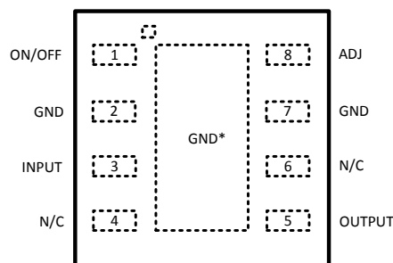
Figure 3. Top View See Package Number NGN
