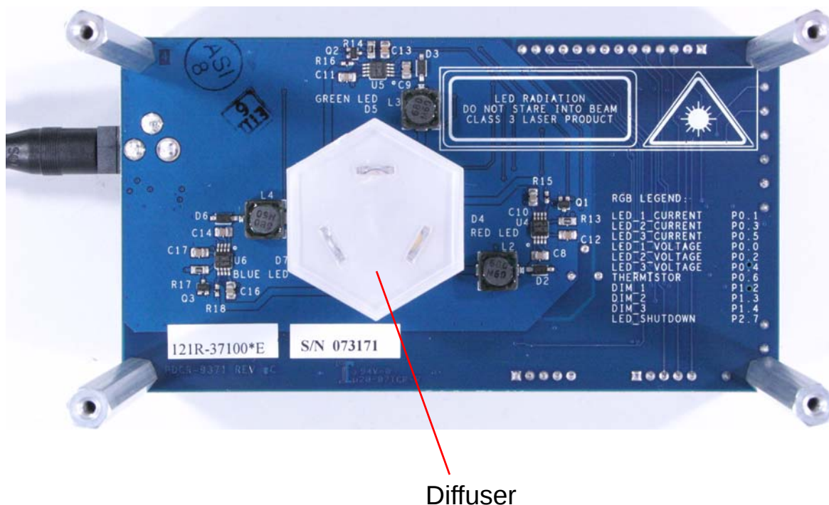
Figure 1-1. Demonstration Board, LED Side
