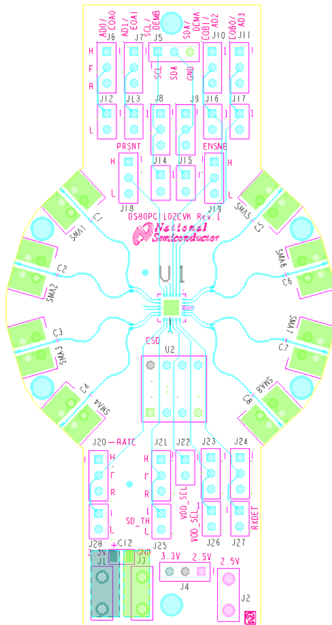
Figure 3: Top Assembly Layer
