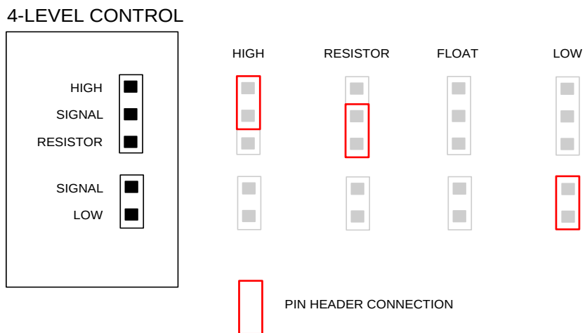
Figure 2: 4-Level IO Control on EVK
