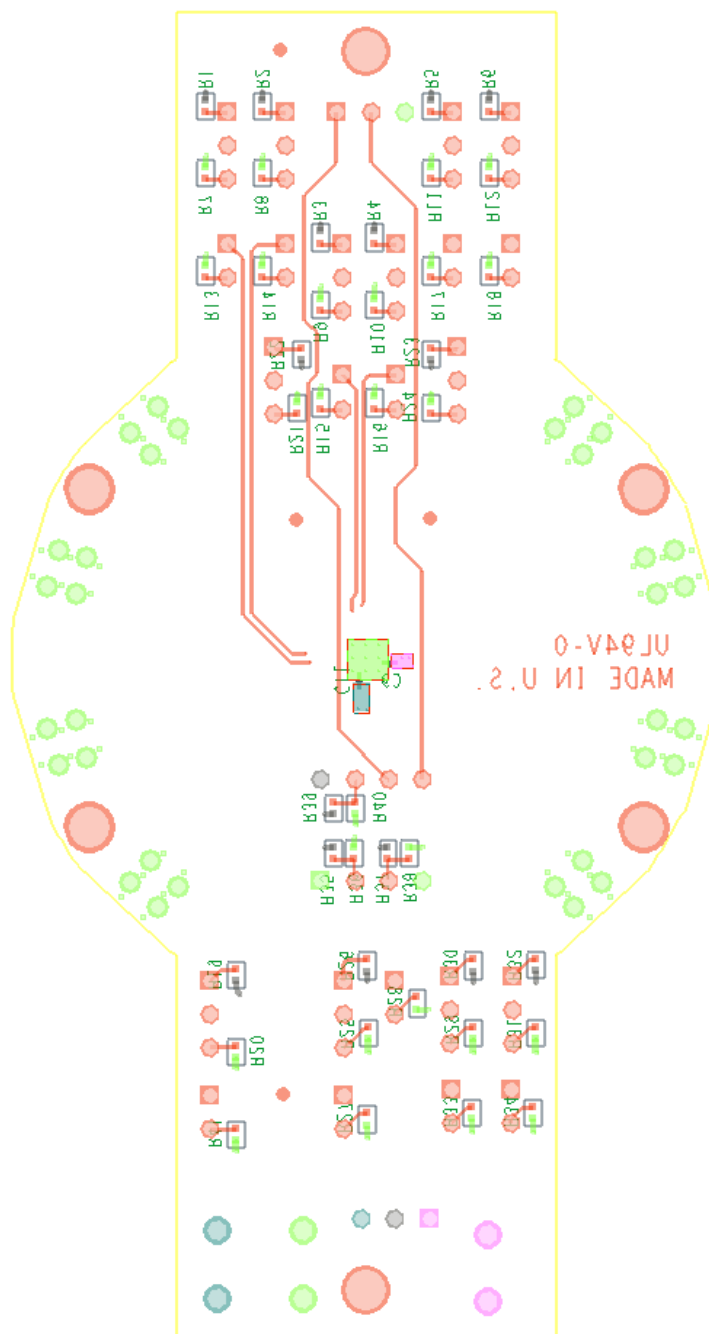
Figure 4: Bottom Assembly Layer
