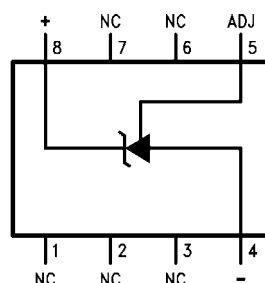
SO Package
