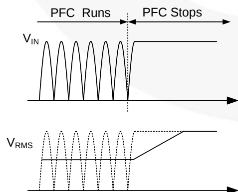
To sense the RMS value of the line voltage, averaging circuit with two poles is typically employed, as shown in Figure 28. Notice that the input voltage of the PFC is clamped at the peak of the line voltage once the PFC stops switching because the junction capacitance of the bridge diode is not discharged, as shown in Figure 31. Therefore, the voltage divider for VRMS should be designed considering the brownout protection trip-point and minimum operation line voltage.
