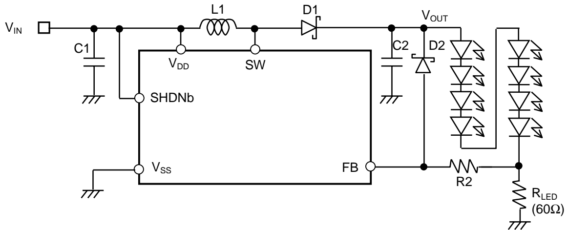
(1) 8 white LEDs
