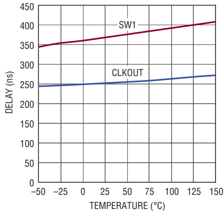
RT/SYNC-to-CLKOUT and SW1 Delay vs Temperature
