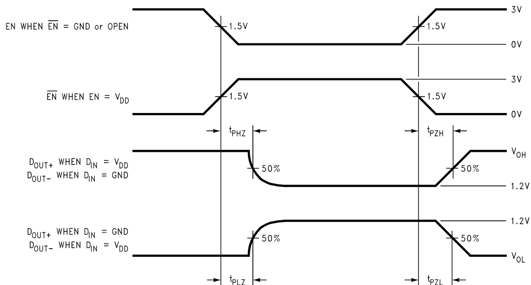
Figure 5. Driver TRI-STATE Delay Waveform
