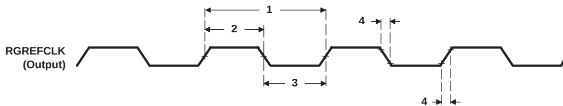
Figure 7-68. RGMIIREFCLK Timing
