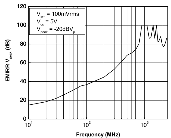
Figure 15. EMIRR vs. frequency at V_{CC} = 5V , T = 25^\circ C
