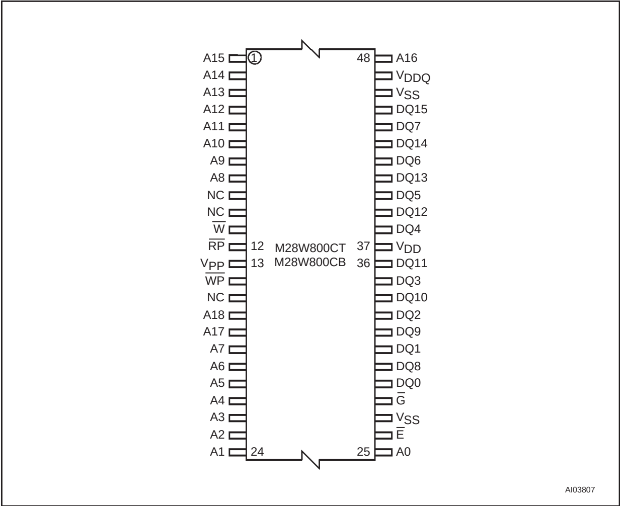
Figure 3. TSOP Connections
