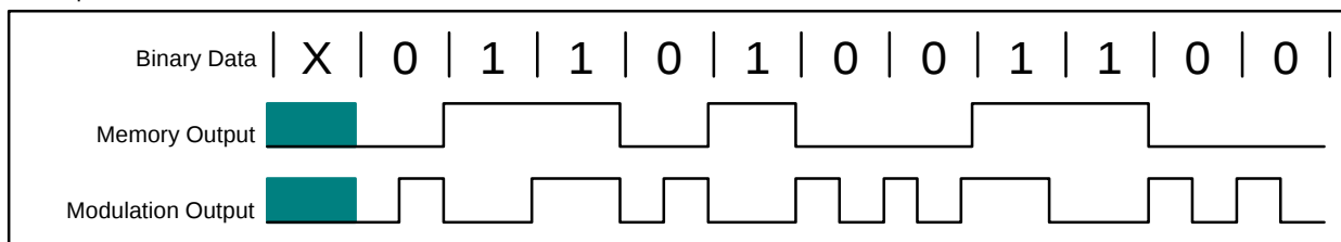
Biphase Code
