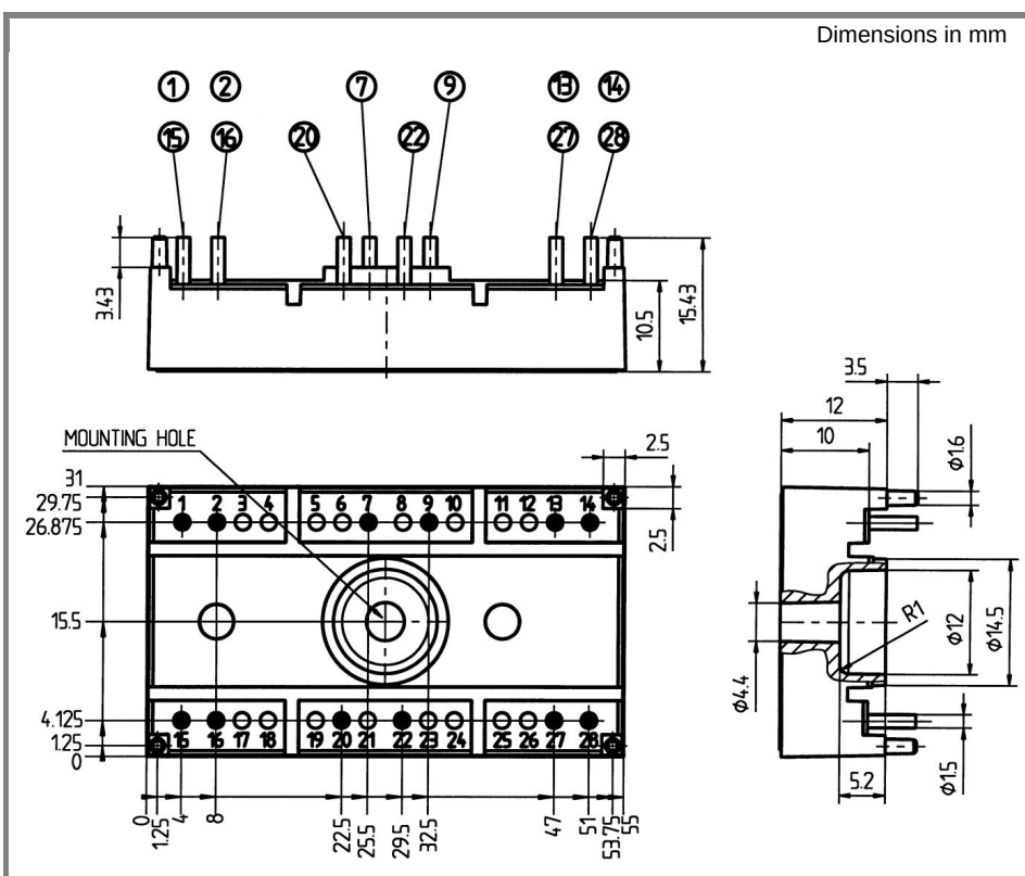
Case T13 (Suggested hole diameter in the PCB for solder pins and mounting pins : 2mm)
