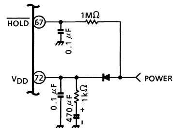
Example of a Condenser Back-Up Circuit
