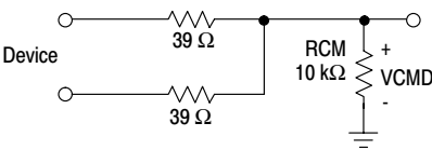
Figure 5. Test Load B3
