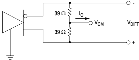
Figure 6. AUI Common Mode Termination
