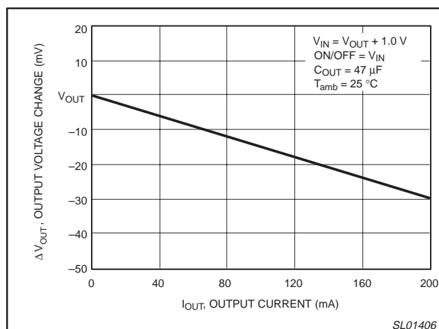
Figure 12. Normalized load regulation.
