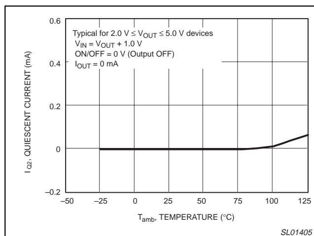
Figure 14. Quiescent current versus temperature.
