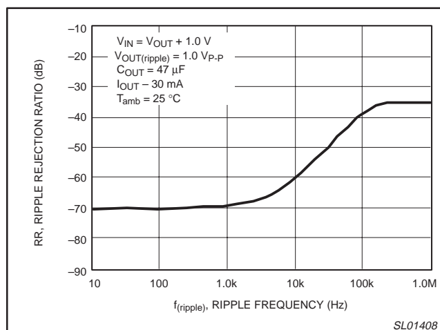
Figure 10. Ripple rejection ratio versus frequency.
