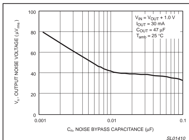
Figure 11. Output noise versus noise capacitance.
