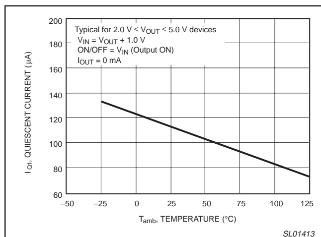
Figure 15. Quiescent current versus temperature.
