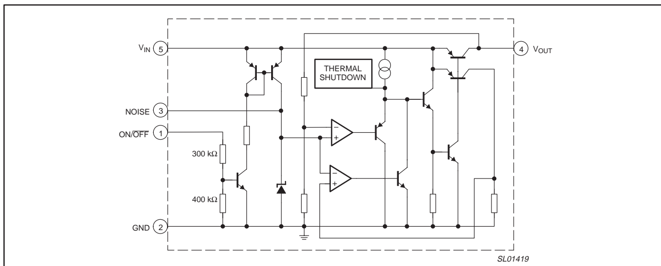
Figure 22. Functional diagram.
