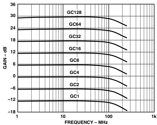
TPC 3. AC Response vs. Gain Control
