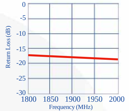
Return Loss vs. Frequency OUTPUT
