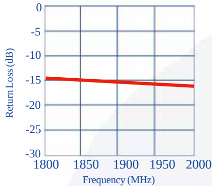
Return Loss vs. Frequency INPUT
