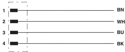
Contact assignment of 7/8" plug
