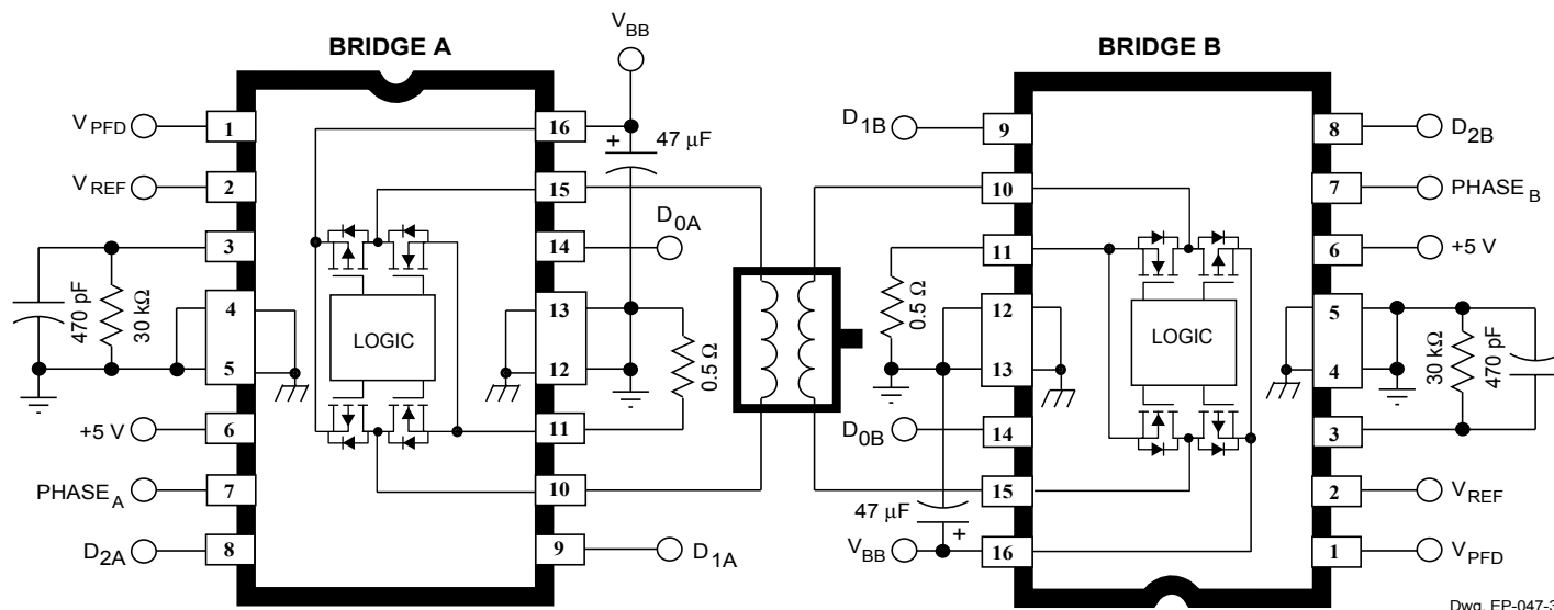
Figure 4 — Typical Application
