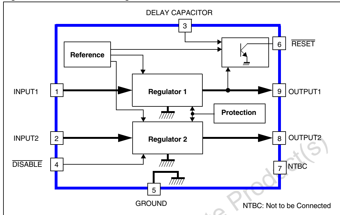
Figure 2. TDA8133 block diagram
