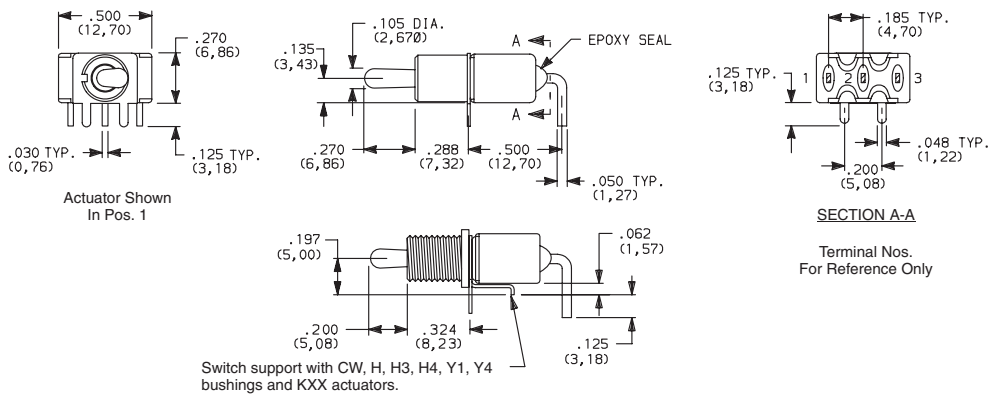
7101MD9ABE Horizontal Actuation SPDT
