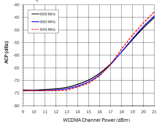
ACP versus WCDMA Channel Power (25C)
