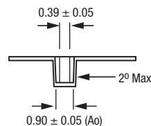
Section A
