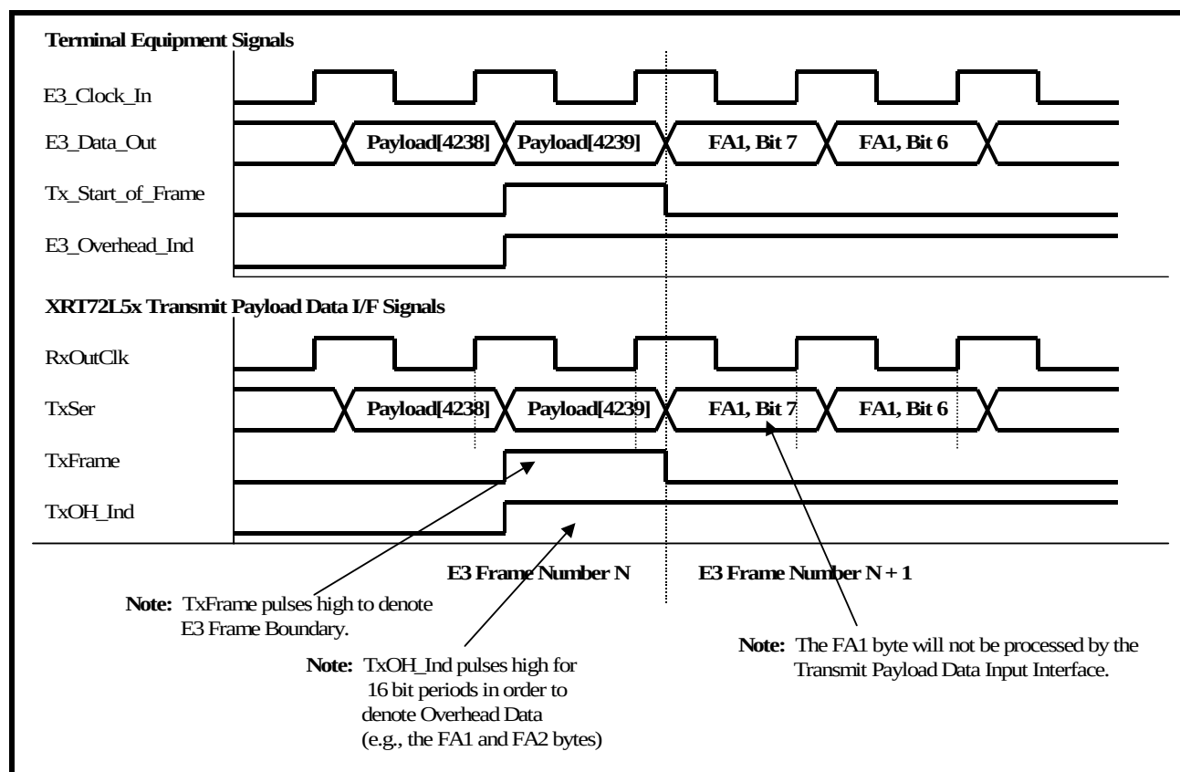
FIGURE 145. BEHAVIOR OF THE TERMINAL INTERFACE SIGNALS BETWEEN THE TRANSMIT PAYLOAD DATA INPUT INTERFACE BLOCK OF THE XRT72L52 AND THE TERMINAL EQUIPMENT (FOR MODE 1 OPERATION)
