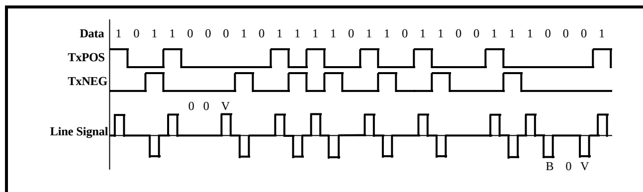
FIGURE 56. ILLUSTRATION OF TWO EXAMPLES OF B3ZS ENCODING
