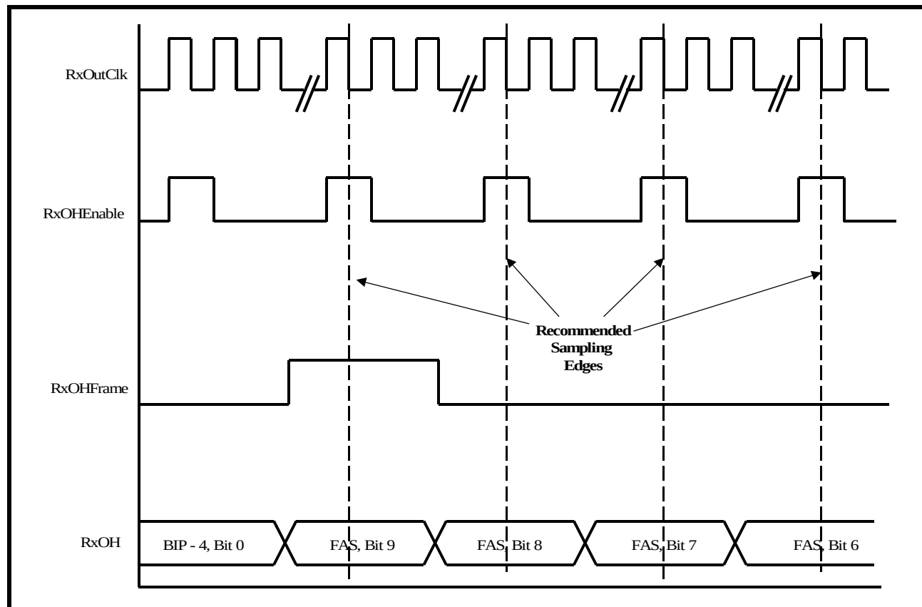
FIGURE 135. ILLUSTRATION OF THE SIGNALS THAT ARE OUTPUT VIA THE RECEIVE OVERHEAD DATA OUTPUT INTERFACE BLOCK (FOR METHOD 2).
