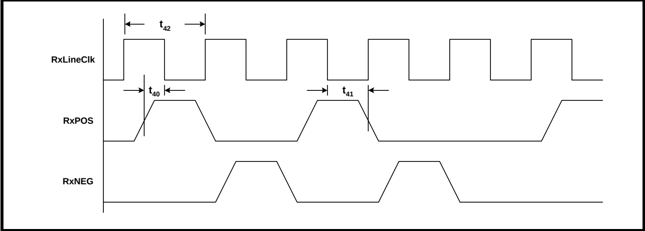
FIGURE 121. WAVEFORM/TIMING RELATIONSHIP BETWEEN RxLINECLK, RxPOS AND RxNEG - WHEN RxPOS AND RxNEG ARE TO BE SAMPLED ON THE FALLING EDGE OF RxLINECLK
