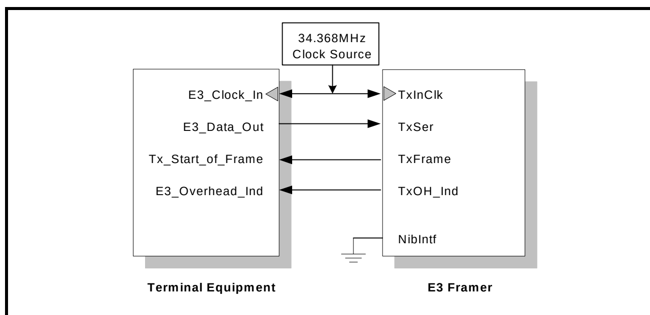
FIGURE 148. THE TERMINAL EQUIPMENT BEING INTERFACED TO THE TRANSMIT PAYLOAD DATA INPUT INTERFACE BLOCK FOR MODE 3 (SERIAL/LOCAL-TIMED/FRAME-MASTER) OPERATION
