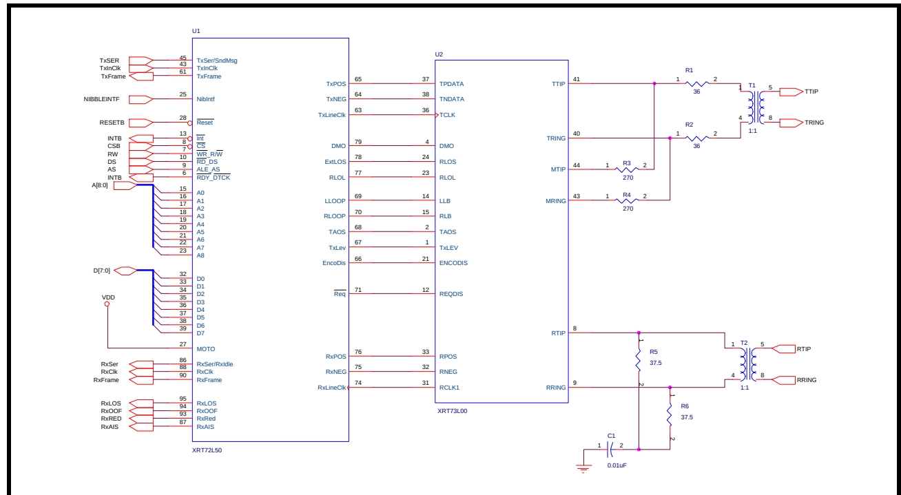
FIGURE 62. IINTERFACING THE XRT72L52 FRAMER IC TO THE XRT73L00 DS3/E3/STS-1 LIU
