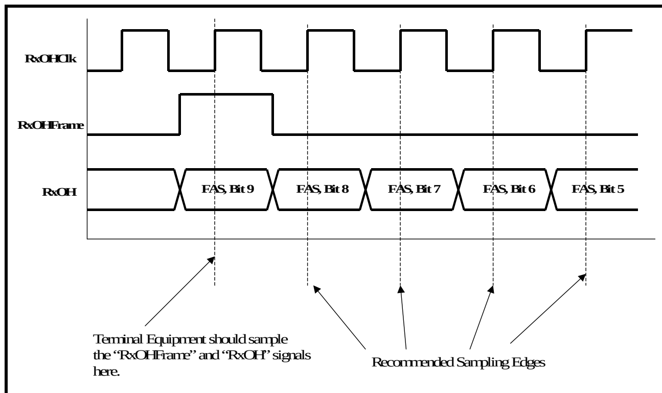
FIGURE 133. ILLUSTRATION OF THE SIGNALS THAT ARE OUTPUT VIA THE RECEIVE OVERHEAD OUTPUT INTERFACE (FOR METHOD 1).
