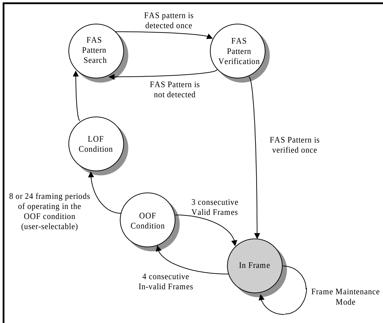
FIGURE 123. THE STATE MACHINE DIAGRAM FOR THE RECEIVE E3 FRAMER E3 FRAME ACQUISITION/MAINTENANCE ALGORITHM
