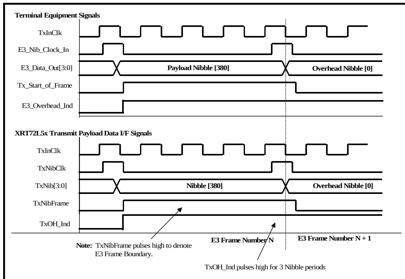
FIGURE 98. BEHAVIOR OF THE TERMINAL INTERFACE SIGNALS BETWEEN THE XRT72L52 AND THE TERMINAL EQUIPMENT (E3 MODE 6 OPERATION)
