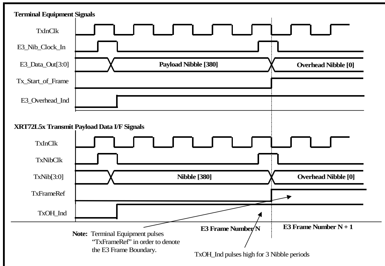
FIGURE 96. BEHAVIOR OF THE TERMINAL INTERFACE SIGNALS BETWEEN THE XRT72L52 AND THE TERMINAL EQUIPMENT (E3, MODE 5 OPERATION)
