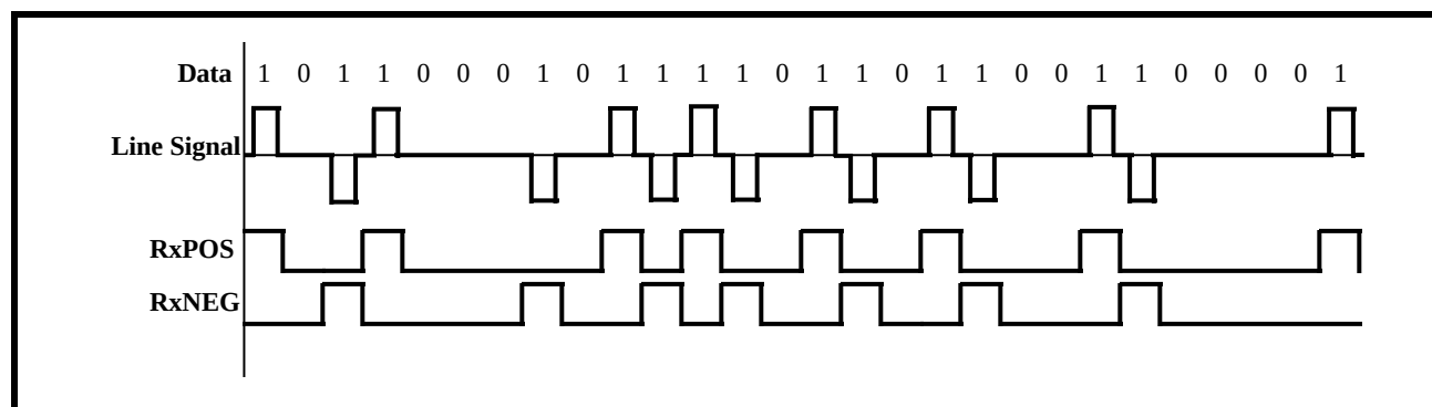
FIGURE 176. ILLUSTRATION OF AMI LINE CODE
