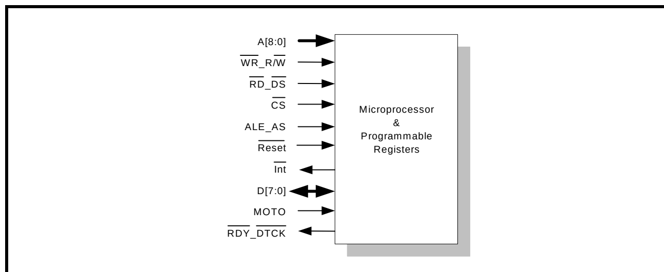
FIGURE 21. BLOCK DIAGRAM OF THE MICROPROCESSOR INTERFACE BLOCK
