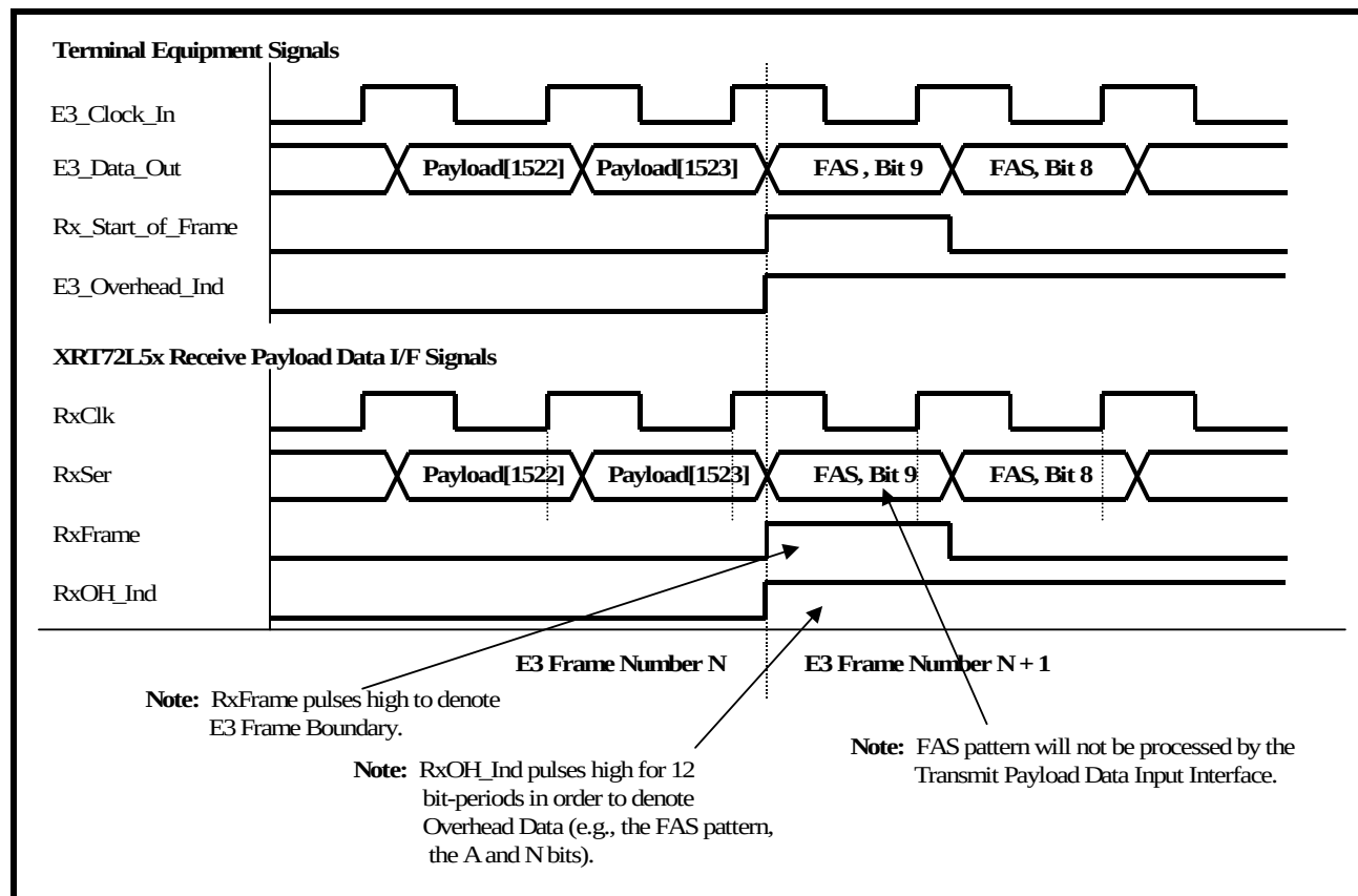
FIGURE 138. AN ILLUSTRATION OF THE BEHAVIOR OF THE SIGNALS BETWEEN THE RECEIVE PAYLOAD DATA OUTPUT INTERFACE BLOCK OF THE XRT72L52 AND THE TERMINAL EQUIPMENT
