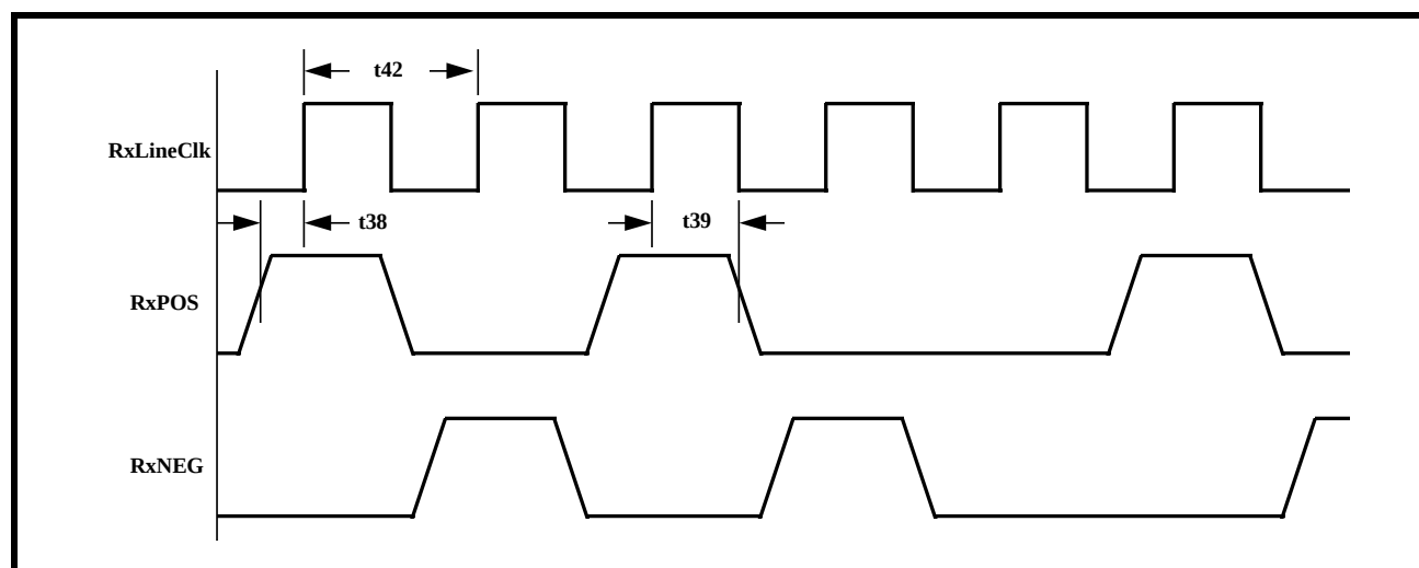
FIGURE 178. WAVEFORM/TIMING RELATIONSHIP BETWEEN RxLINECLK, RxPOS AND RxNEG - WHEN RxPOS AND RxNEG ARE TO BE SAMPLED ON THE RISING EDGE OF RxLINECLK
