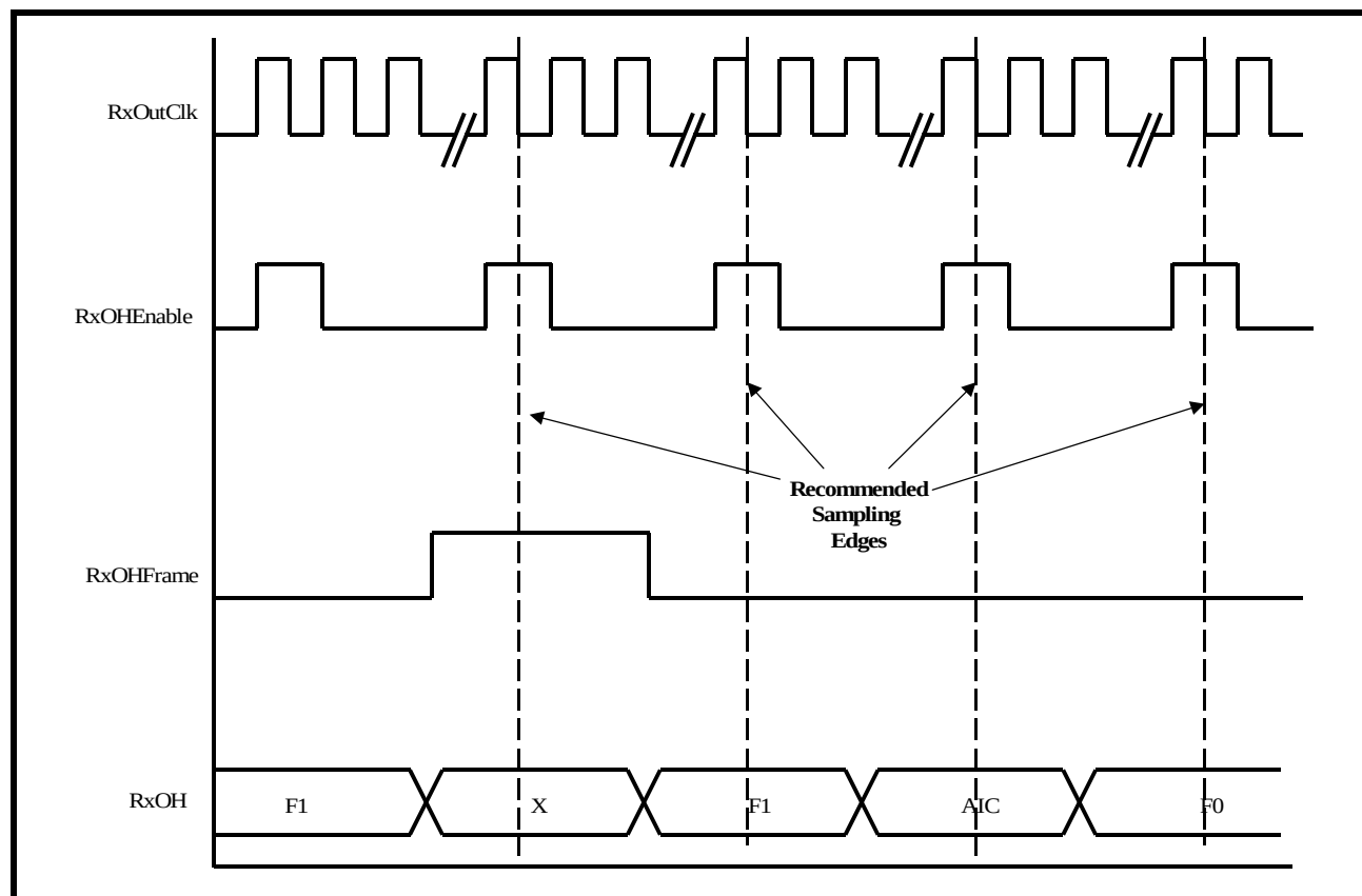
FIGURE 78. ILLUSTRATION OF THE SIGNALS THAT ARE OUTPUT VIA THE RECEIVE OVERHEAD DATA OUTPUT INTERFACE BLOCK (FOR METHOD 2).
