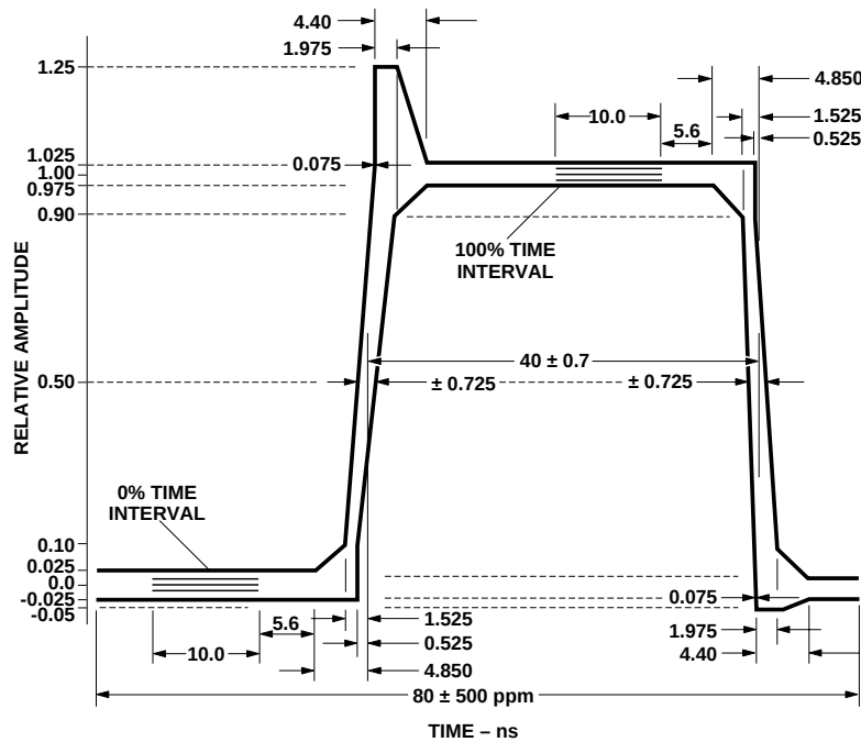
Figure 10. Output Optical Pulse Envelope.
