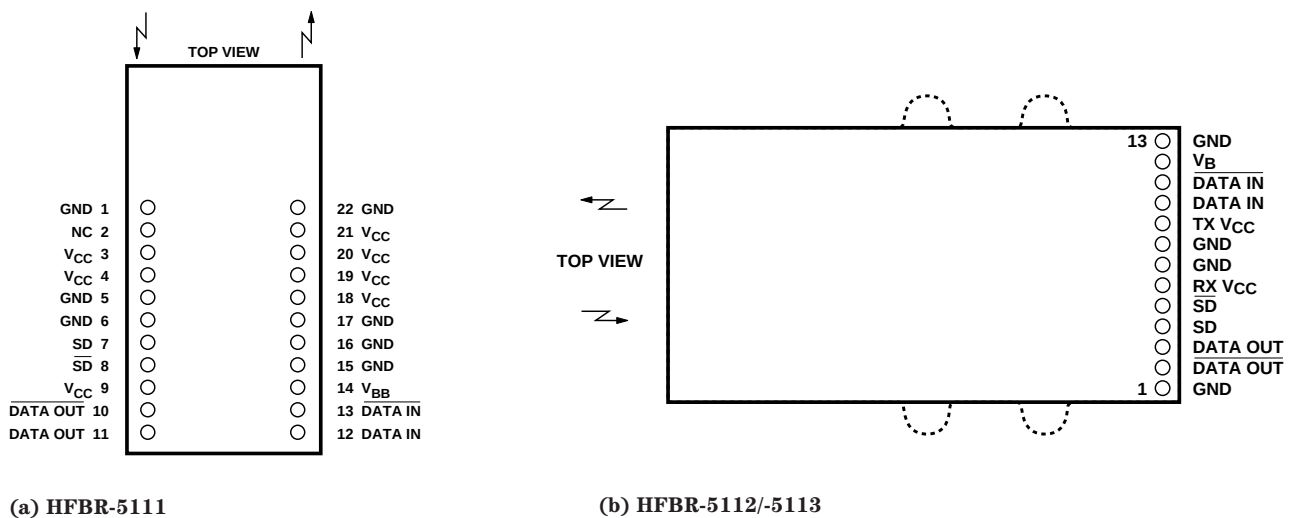
Figure 3. Pin Assignments.
