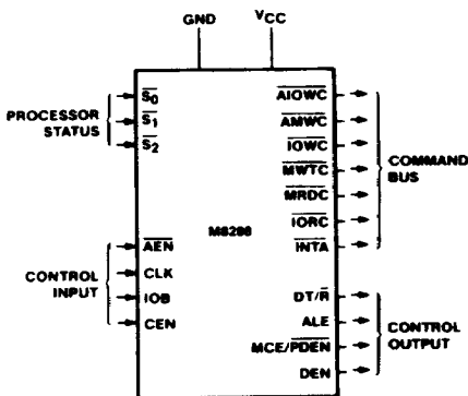
Figure 3. Functional Pin-out
