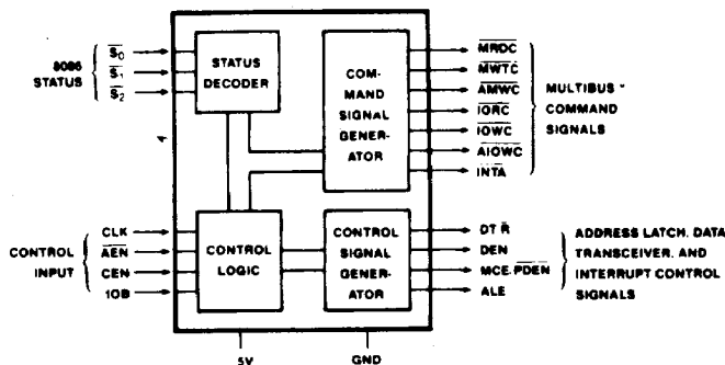
Figure 1. Block Diagram
