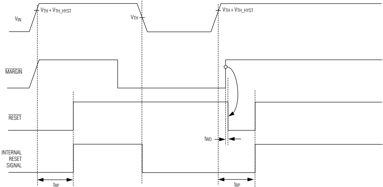
Figure 14. Margin Output Disable ( \overline{\text{MARGIN}} ) Affect on \overline{\text{RESET}} within t_{RP}
