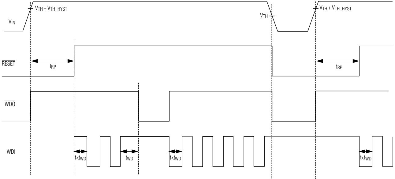
Figure 13. \overline{WDO} Timing Related to V_{TH} and t_{RP}
