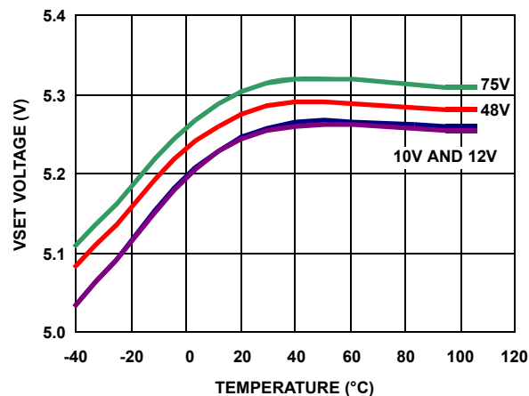
FIGURE 7. VSET VOLTAGE
