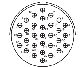
32-31 Service Rating A Number of Contacts 31 Contact Size 16
