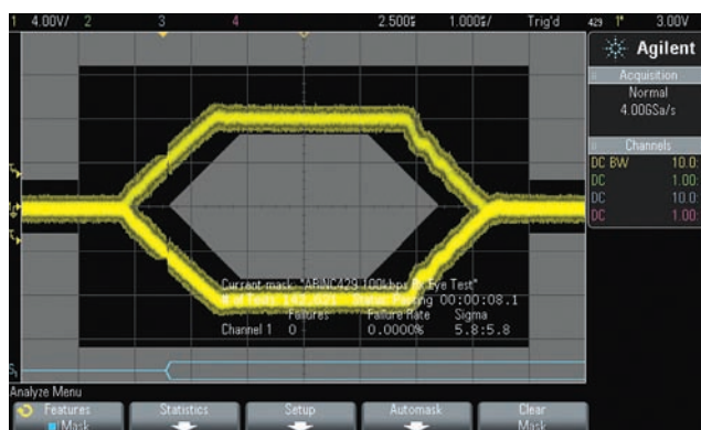
Figure 8: ARINC 429 100 kbps eye-diagram mask test.
