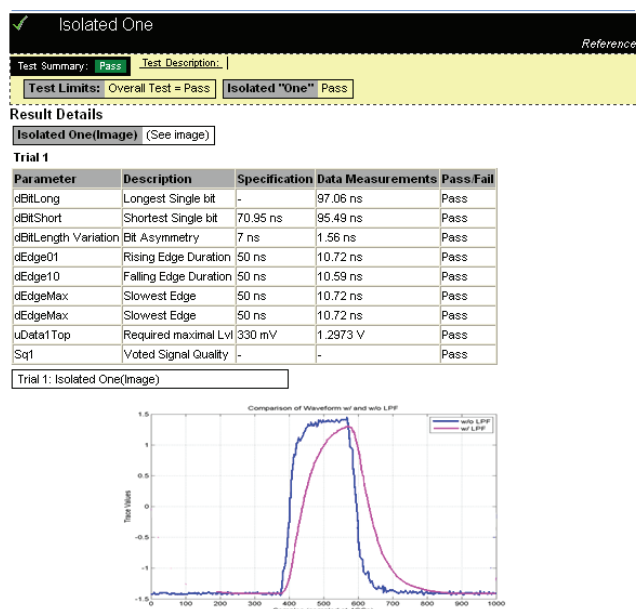
Figure 10: FlexRay signal integrity voting test performed on an isolated "1" bit.
