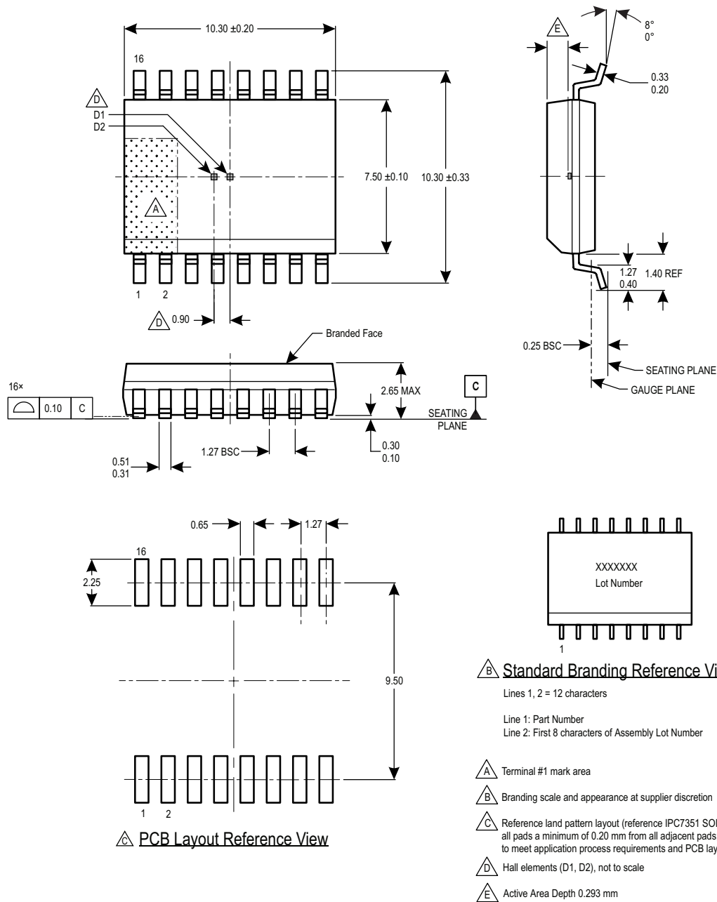
Figure 17: Package MA, 16-Pin SOICW
