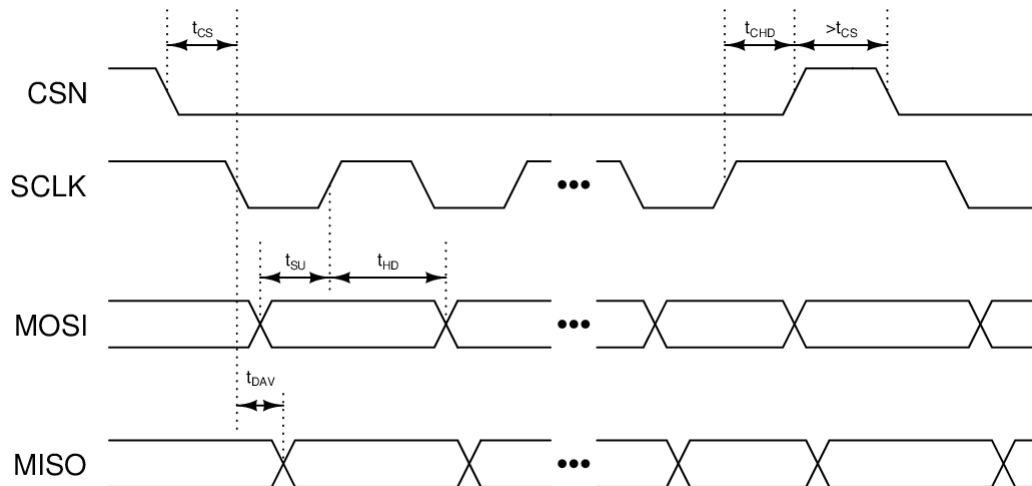
Figure 3: SPI Timing
