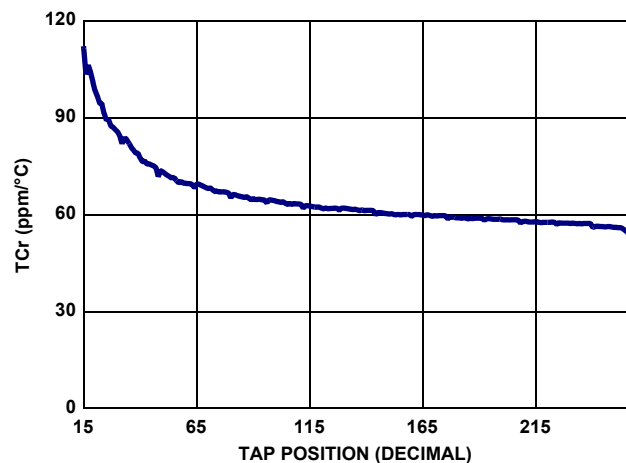
FIGURE 11. 100k TCr vs TAP POSITION
